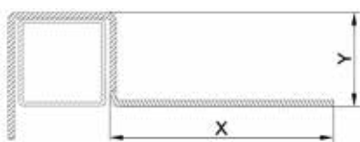
Fixed flange
