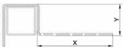
Perforated flange
